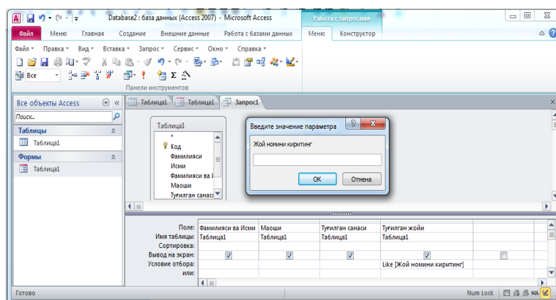
Rasm 5. Parametrlı so'rov yaratish
