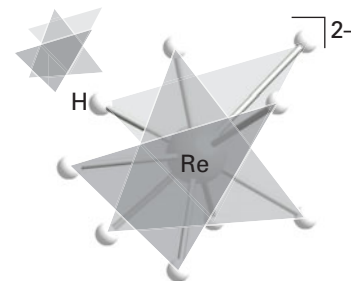
31 [ReH 9 ] 2- ( D_{3h} )
