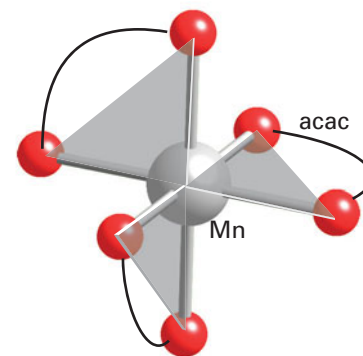
13 [Mn(acac)_3] ( D_3 )
