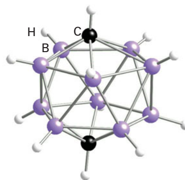
36 closo -1,12- \text{B}_{10}\text{C}_2\text{H}_{12}
