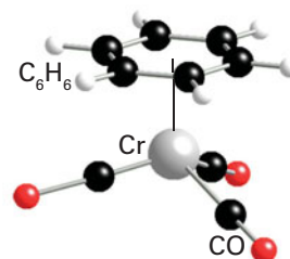
73 [\text{Cr}(\eta^6\text{-C}_6\text{H}_6)(\text{CO})_3]
