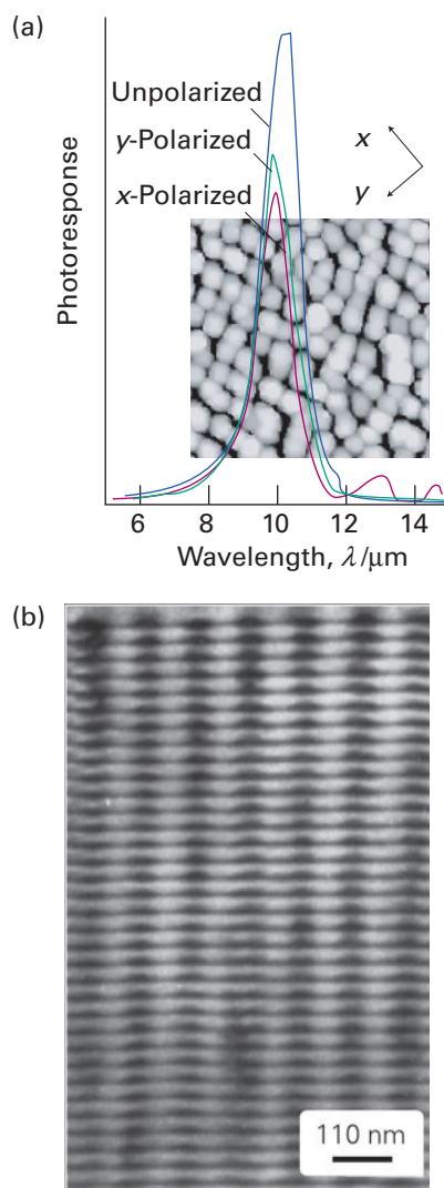
Figure 25.9 (a) Photoresponse (in arbitrary units) of (\text{In}_{0.2}\text{Ga}_{0.8})\text{As} quantum dots formed using MBE. The IR absorption band arises from intraband absorption. The inset is an AFM image of the quantum dots. The quantum dots vary in lateral dimensions between 15 and 20 nm and in vertical height in the range 3–7 nm. (b) A cross-sectional TEM micrograph of an ordered superlattice of (\text{In}_{0.2}\text{Ga}_{0.8})\text{As} quantum dots in a GaAs matrix. (Courtesy of E. Towe.)
