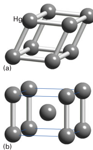
Fig 3.24 The structures of (a) \alpha -mercury and (b) \beta -mercury that are closely related to the unit cells with primitive cubic and body-centred cubic lattices, respectively.
