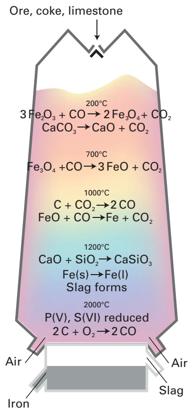
Fig. 5.17 A schematic diagram of a blast furnace showing the typical composition and temperature profile.
