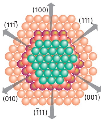
Figure 26.18 Some possible metal crystal planes that might be exposed on a metal surface to a reactive gas. The planes labelled [\bar{1}\bar{1}1] , [1\bar{1}\bar{1}] , etc. are hexagonally close-packed and the planes represented by [100] , [010] , etc. have square arrays of atoms.
