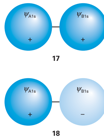
Figure 6.22 The three a_1 molecular orbitals of \text{NH}_3 as computed by molecular modelling software.
