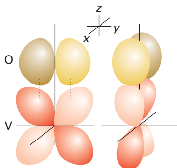
Figure 19.10 The d–p π-bonding between O and V in the vanadyl group VO 2+ . It is convenient to think of the O as having oxidation number –2 and V as +4. Thus, both electron pairs for the two π bonds are donated from the O 2- ion into the metal d yz and d xz orbitals.
