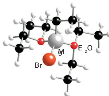
12 \text{MgBr}(\text{OEt}_2)_2
