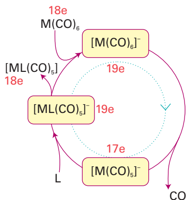
Figure 22.17 Schematic diagram of an electron transfer catalysed CO substitution. After addition of a small amount of a reducing initiator, the cycle continues until the limiting reagent M(CO)_6 or L has been consumed.
