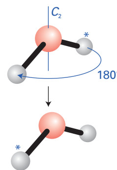
Figure 6.1 An H 2 O molecule may be rotated through any angle about the bisector of the HOH bond angle, but only a rotation of 180° (the C 2 operation) leaves it apparently unchanged.
