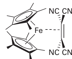
6 [(\eta^5\text{-Cp}^*)_2\text{Fe}(\text{TCNE})]
