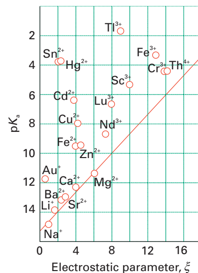
Figure 4.5 The correlation between acidity constant and the electrostatic parameter \xi of aqua ions.
