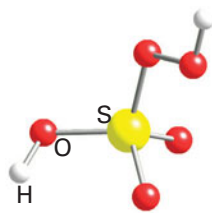
28 Peroxomonosulfuric acid, \text{H}_2\text{SO}_5
