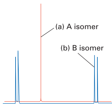
Figure 7.5 Idealized ^{31}P -NMR spectra of two isomers of [PtBrCl(PR_3)_2] . The fine structure due to Pt is not shown.
