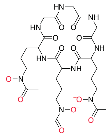
18 Ferrichrome
