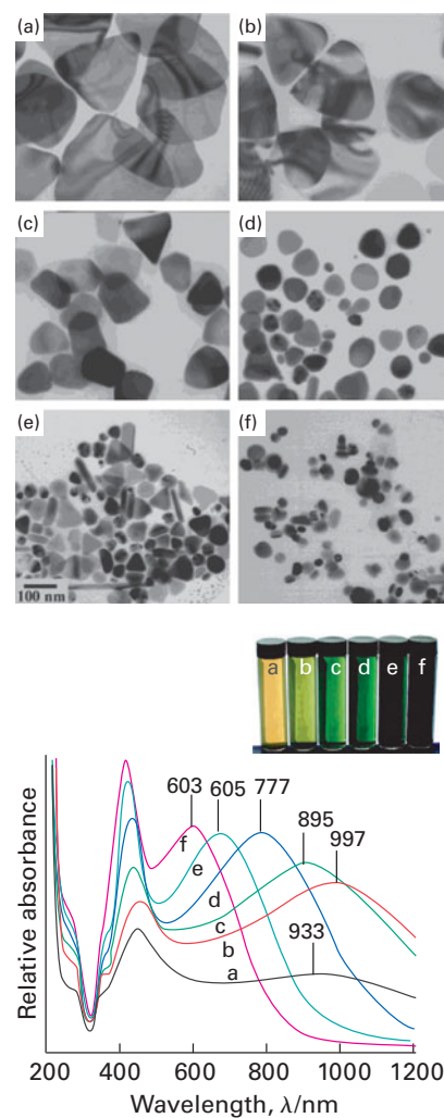
Figure 25.1 (Top) TEM images of the silver nanoplates obtained with different seed amounts: (a) 0.1 \text{ cm}^3 , (b) 0.25 \text{ cm}^3 , (c) 0.5 \text{ cm}^3 , (d) 1.0 \text{ cm}^3 , (e) 2.0 \text{ cm}^3 , and (f) 3.0 \text{ cm}^3 . (Bottom) Absorption spectra of the corresponding silver nanoplate solutions. (S. Chen and D.L. Carroll, J. Phys. Chem. B , 2004, 108 , 5500.)
