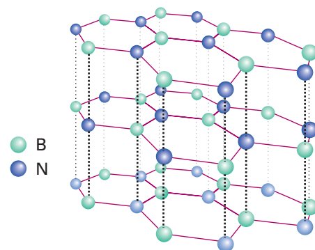
Figure 13.4 The structure of layered hexagonal boron nitride. Note that the rings are in register between layers.
