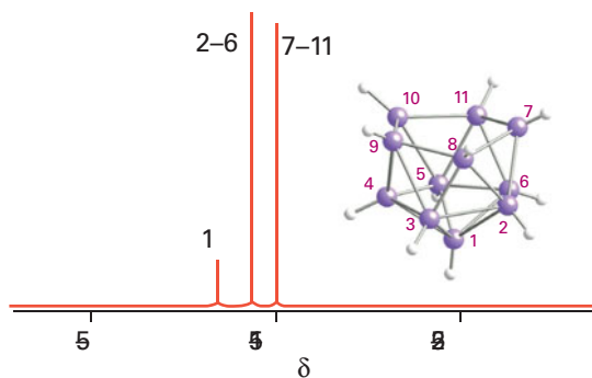
Figure 13.13 The proton-decoupled ^{11}\text{B} -NMR spectrum of [B_{11}H_{14}]^- . The nido structure (a truncated icosahedron) is indicated by the 1:5:5 pattern.
