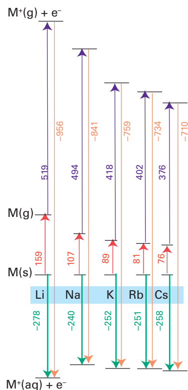
Figure 11.3 Thermochemical cycle (standard enthalpy changes in \text{kJ mol}^{-1} ) for the oxidation half-reaction \text{M}(\text{s}) \rightarrow \text{M}^+(\text{aq}) + \text{e}^- .
