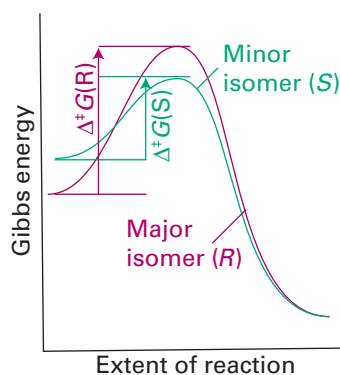
Figure 26.6 Kinetically controlled stereoselectivity. Note that \Delta^+G_S < \Delta^+G_R , so the minor isomer reacts faster than the major isomer.
