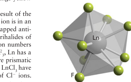
1 Ln coordination in LnF 3
