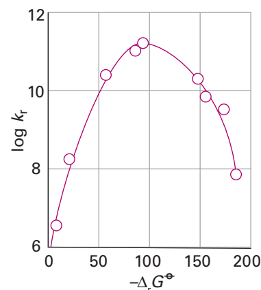
Figure 21.21 Plot of \log_{10} k_r against -\Delta_r G^\ominus for the iridium complex (20) in acetonitrile solution at room temperature. The rates are for electron transfer from the photoexcited \text{Ir}_2 unit to the outlying pyridinium functionalities. (Data from L.S. Fox, M. Kozik, J.R. Winkler, and H.B. Gray, Science 1990, 247 , 1069).
