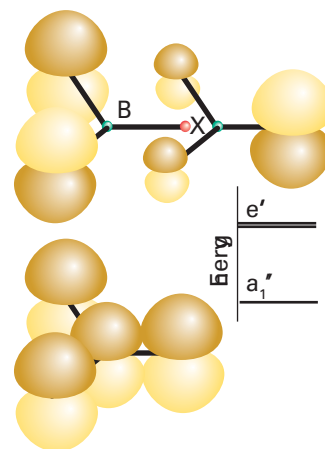
Figure 13.2 The bonding \pi orbitals of boron trihalide are largely localized on the electronegative halogen atoms, but overlap with a p orbital of boron is significant in the a_1' orbital.
