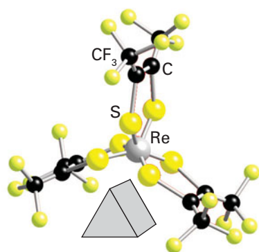
21 [Re(S(CF 3 )C=C(CF 3 )S) 3 ]
