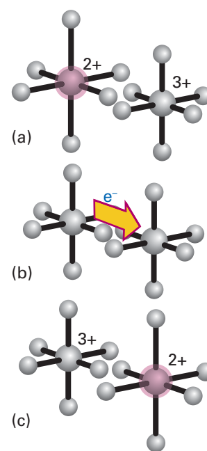
Figure 21.17 Electron transfer between two metal ions in a precursor complex is not productive until their coordination shells have reorganized to be of equal size. (a) Reactants; (b) reactant complexes having distorted into the same geometry; (c) products.
