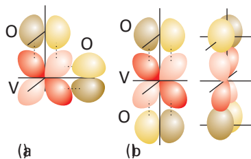
Figure 19.11 Comparison of the competition between cis and trans oxygens attached to vanadium. (a) In the cis configuration the metal has only one d orbital in common with the π orbitals on the O atoms. (b) In the trans configuration the metal atom has two d orbitals in common with the π orbitals on the two O atoms.
