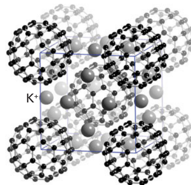
Figure 24.68 The structure of K 6 C 60 with a body-centred cubic unit cell with C 60 6- molecular ions at the cell corners and body centre, and K + ions occupying half of the sites in the faces of the cell which have approximate tetrahedral coordination to four C 60 molecular ions.
