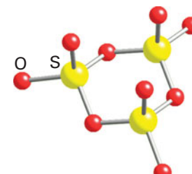
4 (\text{SO}_3)_n, C_{3v}
