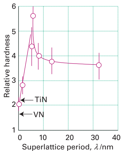
Figure 25.24 The dependence of hardness on the superlattice period for (\text{TiN})_m(\text{VN})_n superlattices. (Adapted from U. Helmersson, et al. , J. Appl. Phys. , 1987, 62, 481.)
