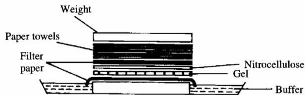
Figure 13.14 The transfer of DNA from a gel to a nitrocellulose sheet. Buffer soaks through the gel to the nitrocellulose and takes the DNA with it.
