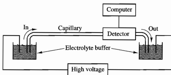
Figure 3.33 Capillary electrophoresis. The sample is introduced through the inlet, washed in with a wash buffer and then separated under the influence of a potential difference between the two electrodes. The zones are monitored as they pass through the detector and the data captured and computed.
