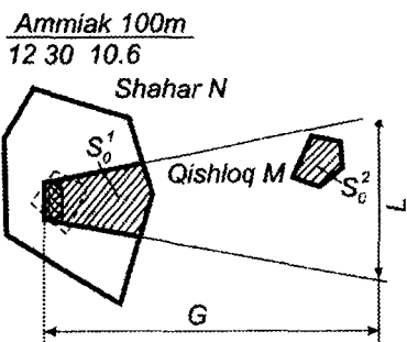
5-rasm. KTZM ta'siridagi avariya kimyoviy shikastlanish o'chog'ining sxemasi
