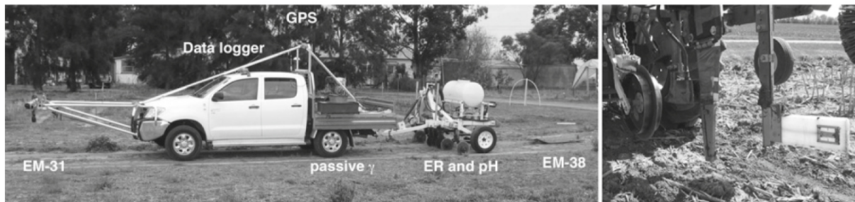
Fig. 9. Multisensor platforms. (left) A multisensor platform with electromagnetic induction, passive gamma-ray spectrometry, electrical resistivity, and pH sensors and (right) one with mechanical, electrical, and optical sensors [after Viscarra Rossel et al. , 2011].
