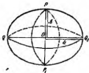
1.2-rasm. Ellipsoid
