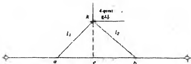
6.3-rasm. Chiziqli kestirma usuli
