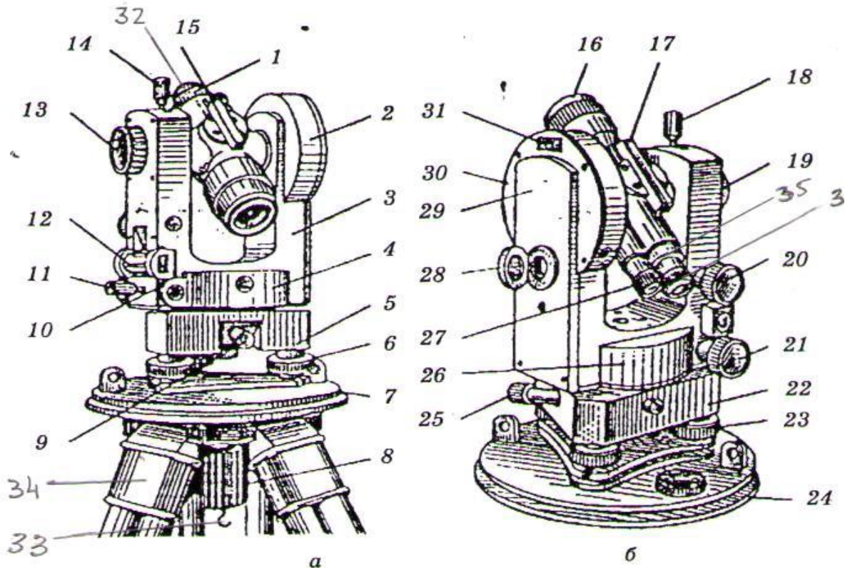
4.2-rasm. T30 teodolit tuzilishi
