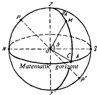
4-rasm. Gorizont koordinatalar sistemasi
