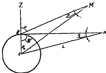
19-rasm. Yoritgichlarning sutkalik va sutkalik-gorizonttal parallakslari
