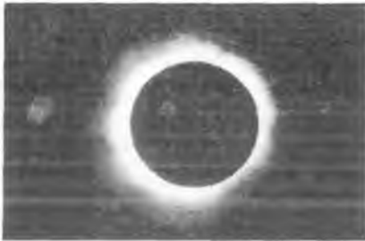
46-rasm. Quyoshning to'la tutilishi
