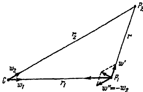
29-rasm. Uch jism masalasida P_1 birinchi sayyora, P_2 ikkinchi sayyoraning beradigan chetlantiruvchi tezlanishi kattaligi
