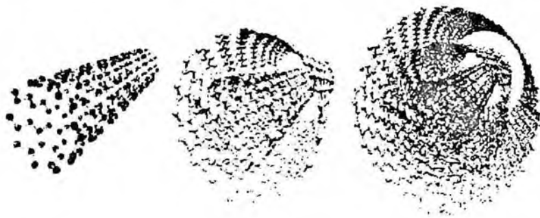
42-rasm. Nanotrubbkalar
