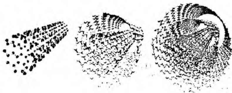
42-rasm. Nanotrubbkalar
