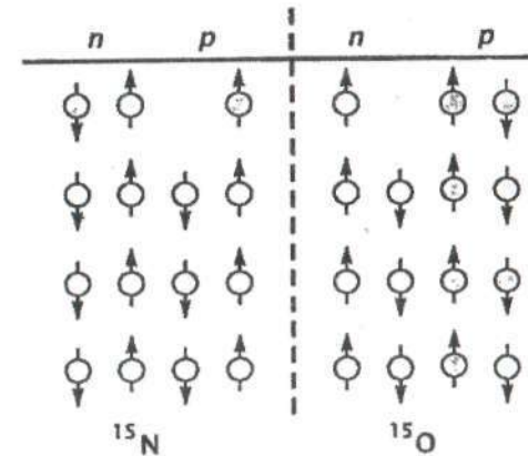
1.3-rasm. Kuzgu yadrolar.
