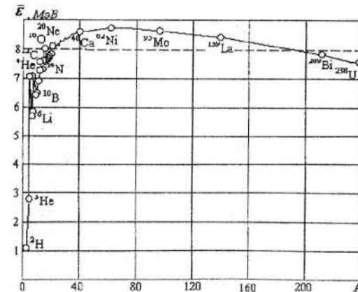
1.5-rasm. Solishtirma bog'lanish energiyasining massa soniga bog'lanishi.
