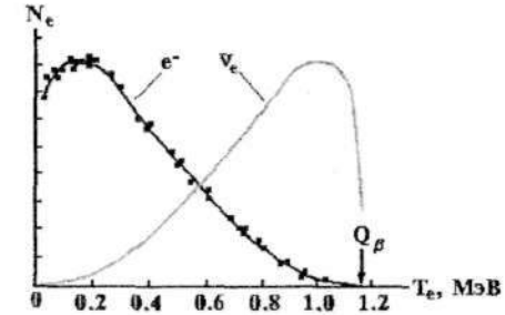
4.5-rasm. {}^{210}_{83}\text{Bi} \rightarrow {}^{210}_{84}\text{Po} + e^- + \bar{\nu}_e parchalanishda hosil bo'ladigan elektron va neytrinolarning energetik spektrlari.
