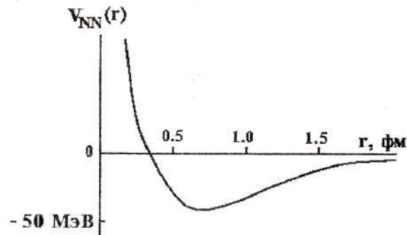
2.1-rasm. Nuklon-nuklon o'zaro ta'sir potentsiali radial bog'lanishi.
