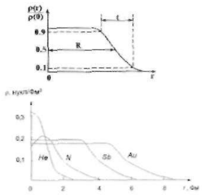
1.6-rasm. Atom yadrosida zaryad taqsimoti.
