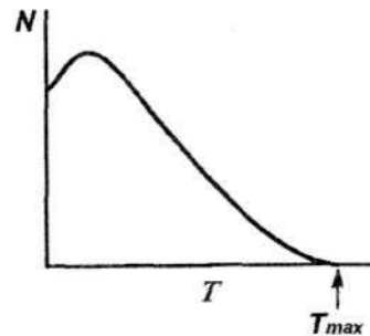
4.4-rasm. Beta-parchalanish spektri.
