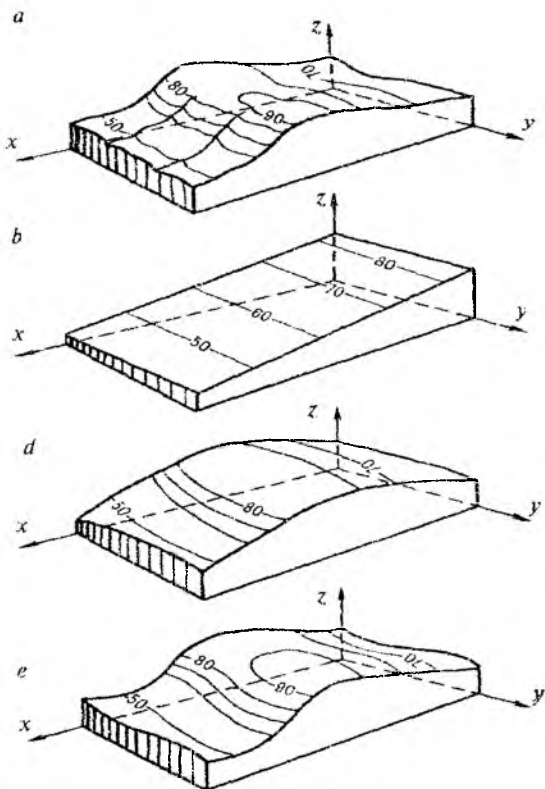
12.15-rasm. Yuзалarni approssimasiyalash (yaqinlashtirish).
